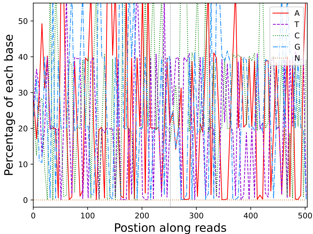
Base percentage along reads (R10301)
